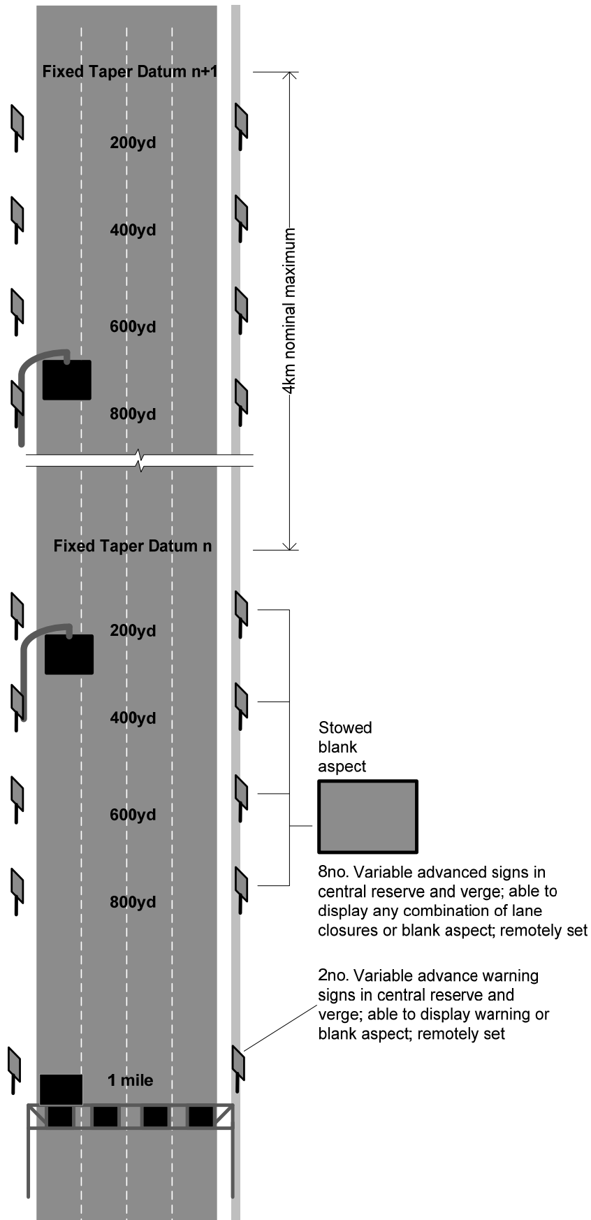
Figure 1: FTP and advanced signs - stowed / not in use
