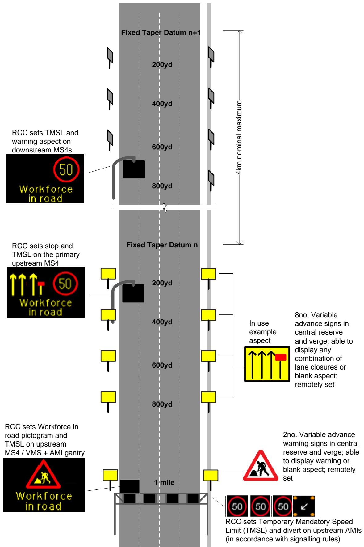
Figure 2: FTP and advance signs set ready for coning to commence for maintenance in Lane 4, 400yd upstream of FTP datum n+1. Note that aspects depicted on electronic scheme signals are indicative only.
